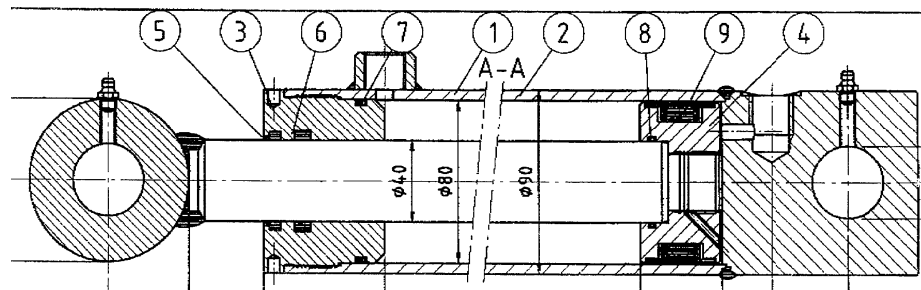
Zylinder 80/40-400 (91825)
