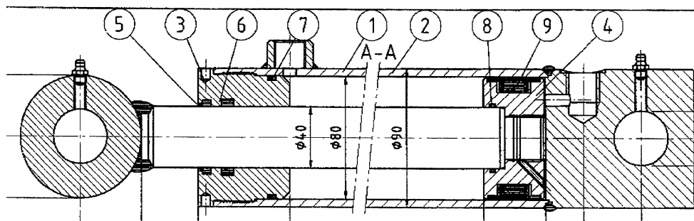
Cylinder 80/40-350 (91805)
